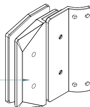
REAR ISOMETRIC VIEW
